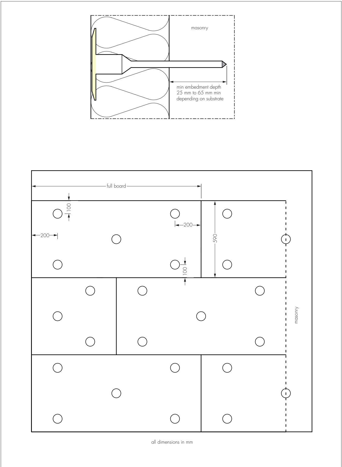
Figure 5 Insulation board fixing pattern
