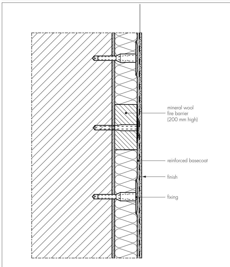
Figure 2 Fire barrier details
