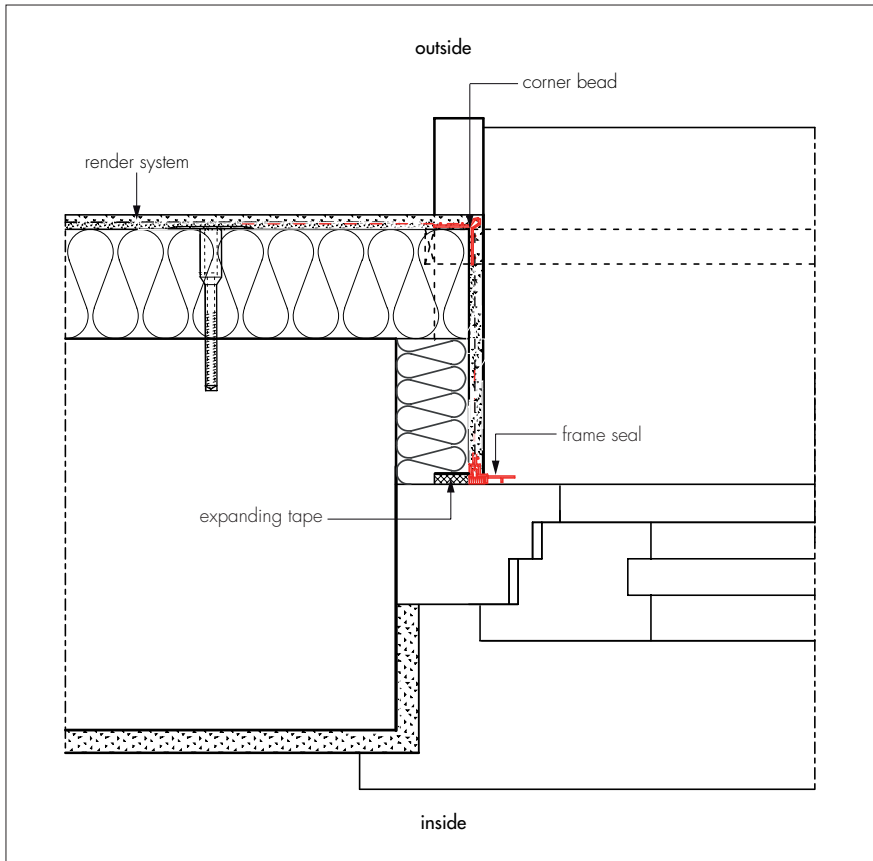
Figure 10 Window reveal
